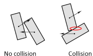
Figure 2.2. Colliding objects
