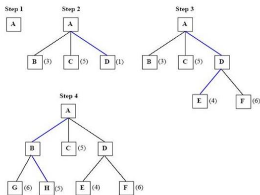
Gambar 2.2 Ilustrasi Algoritma Best First Search
