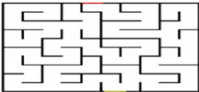
Gambar 3.2 Labirin Original
