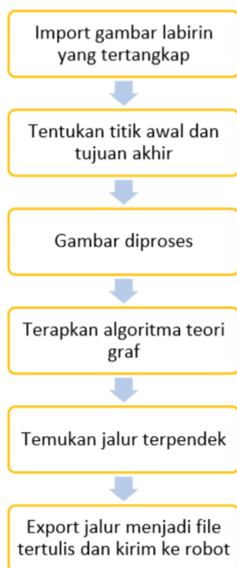
Gambar 3.4 Diagram Alir Program
