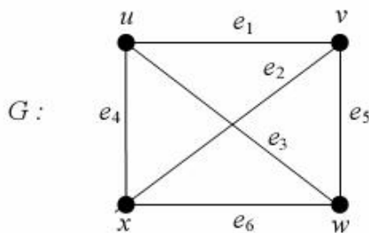
Gambar 2.3 Graf reguler
