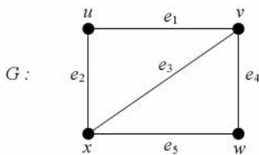
Gambar 2.2 Adjacent dan incident
