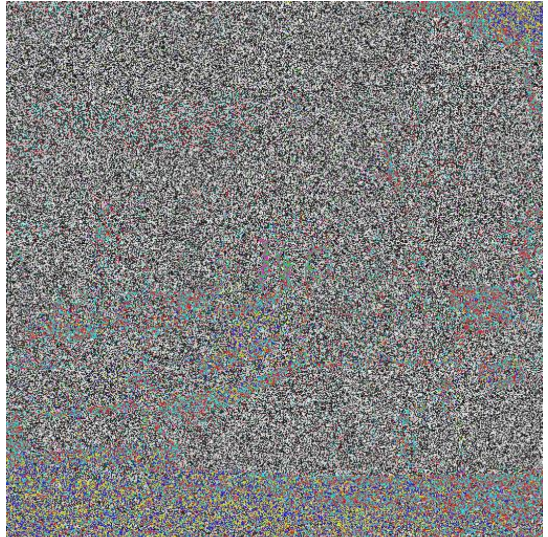
Cipher-image
