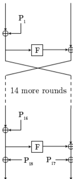
Gambar 2 Struktur Blowfish Cipher
