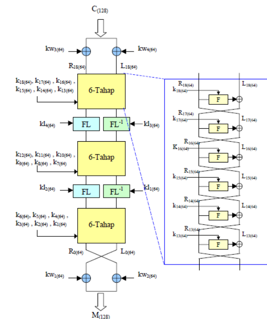
Gambar 7 Dekripsi Camellia Cipher Mode 128 Bit
